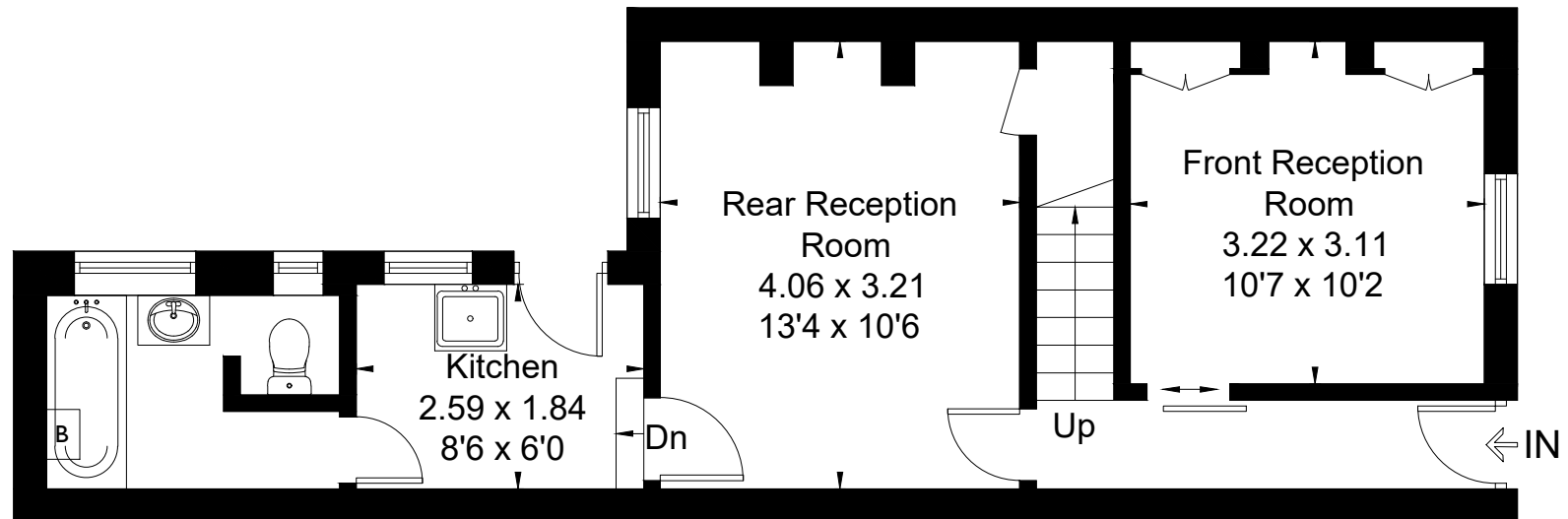
Ground Floor
