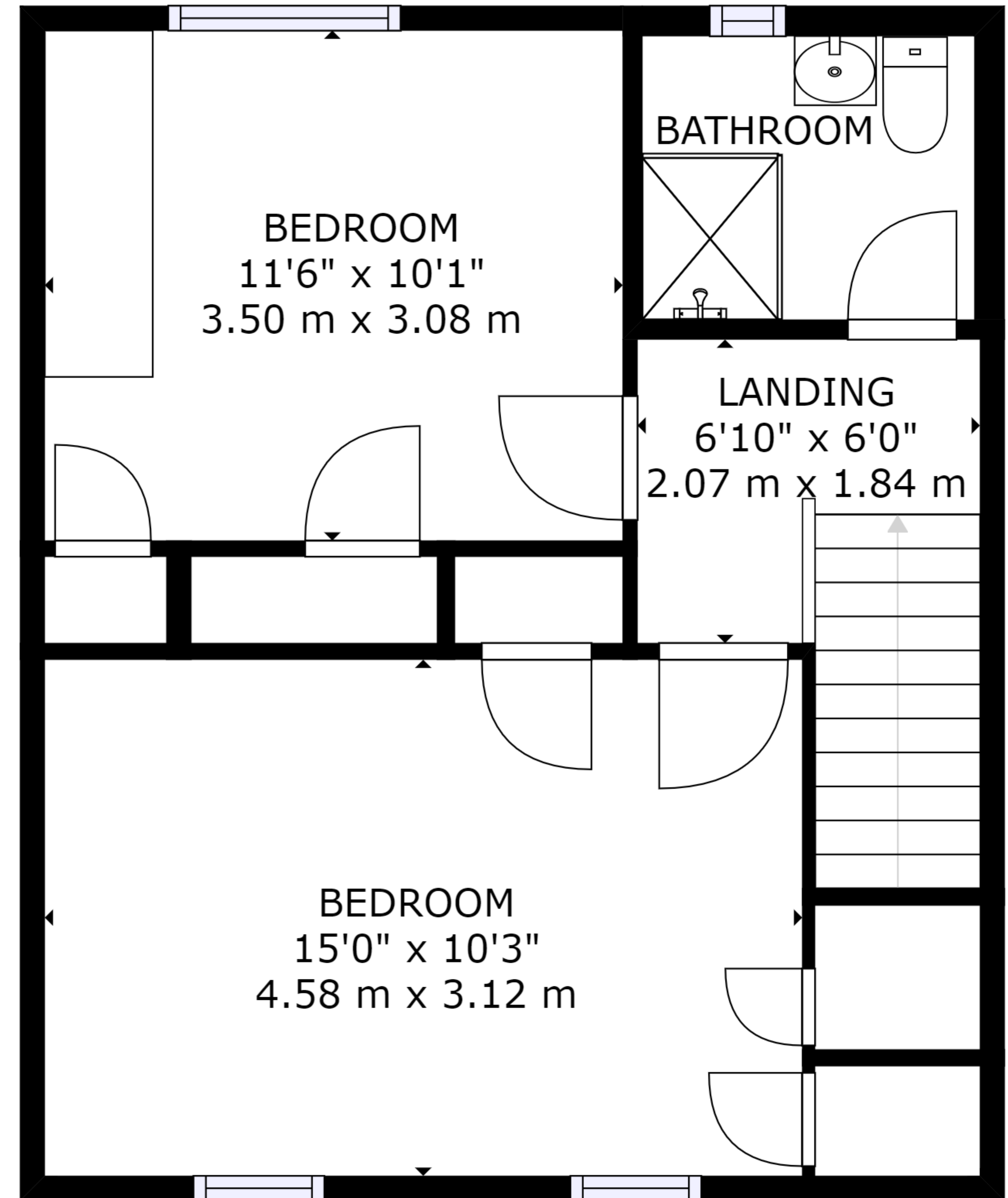
FLOOR 2
