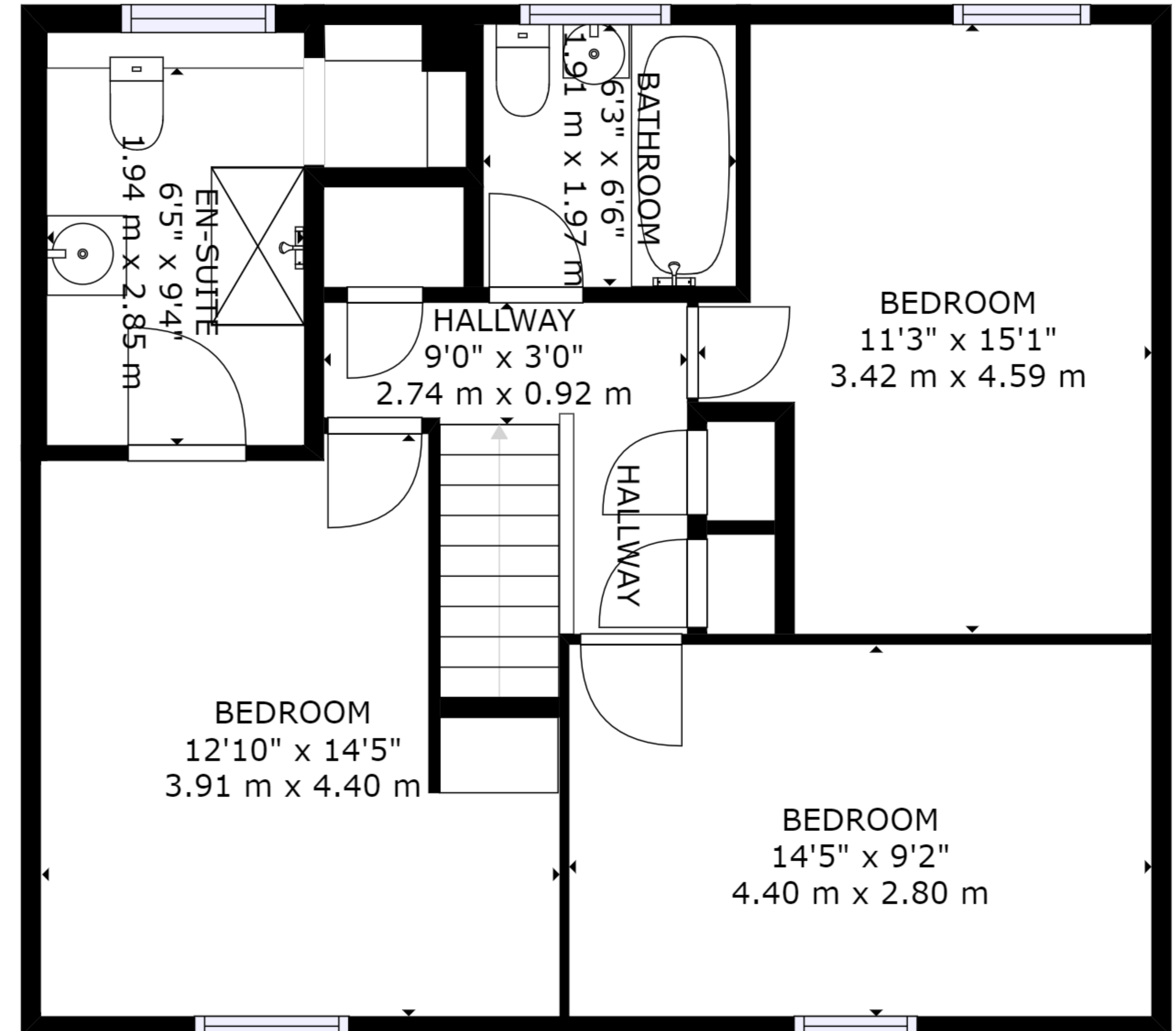
FLOOR 2
