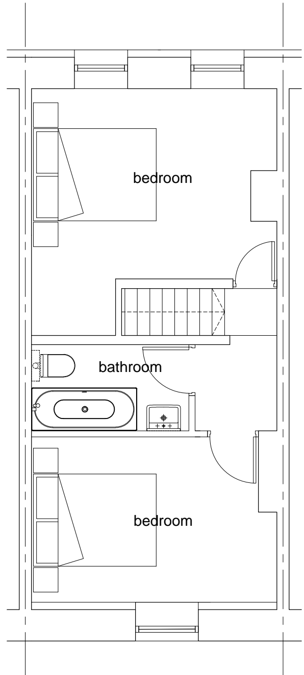
First Floor
