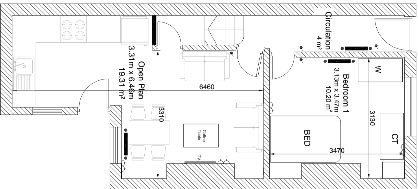
PROPOSED GROUND FLOOR GROSS INTERNAL FLOOR AREA 37 SQ M
