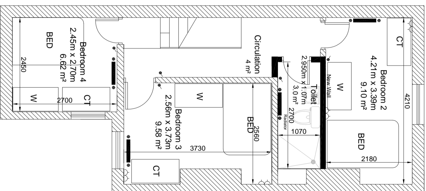
PROPOSED FIRST FLOOR GROSS INTERNAL FLOOR AREA 35 SQ M
