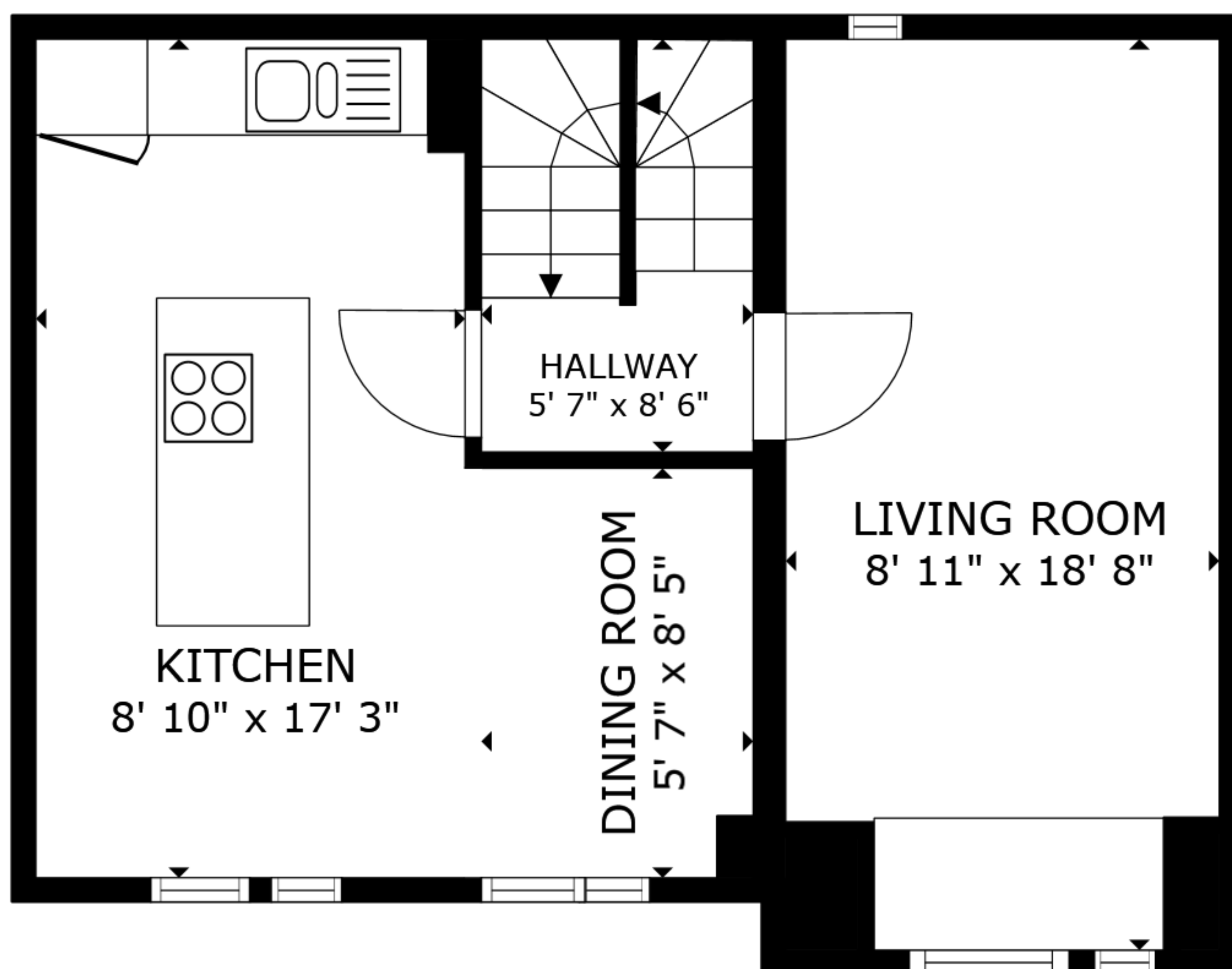
FLOOR 3
