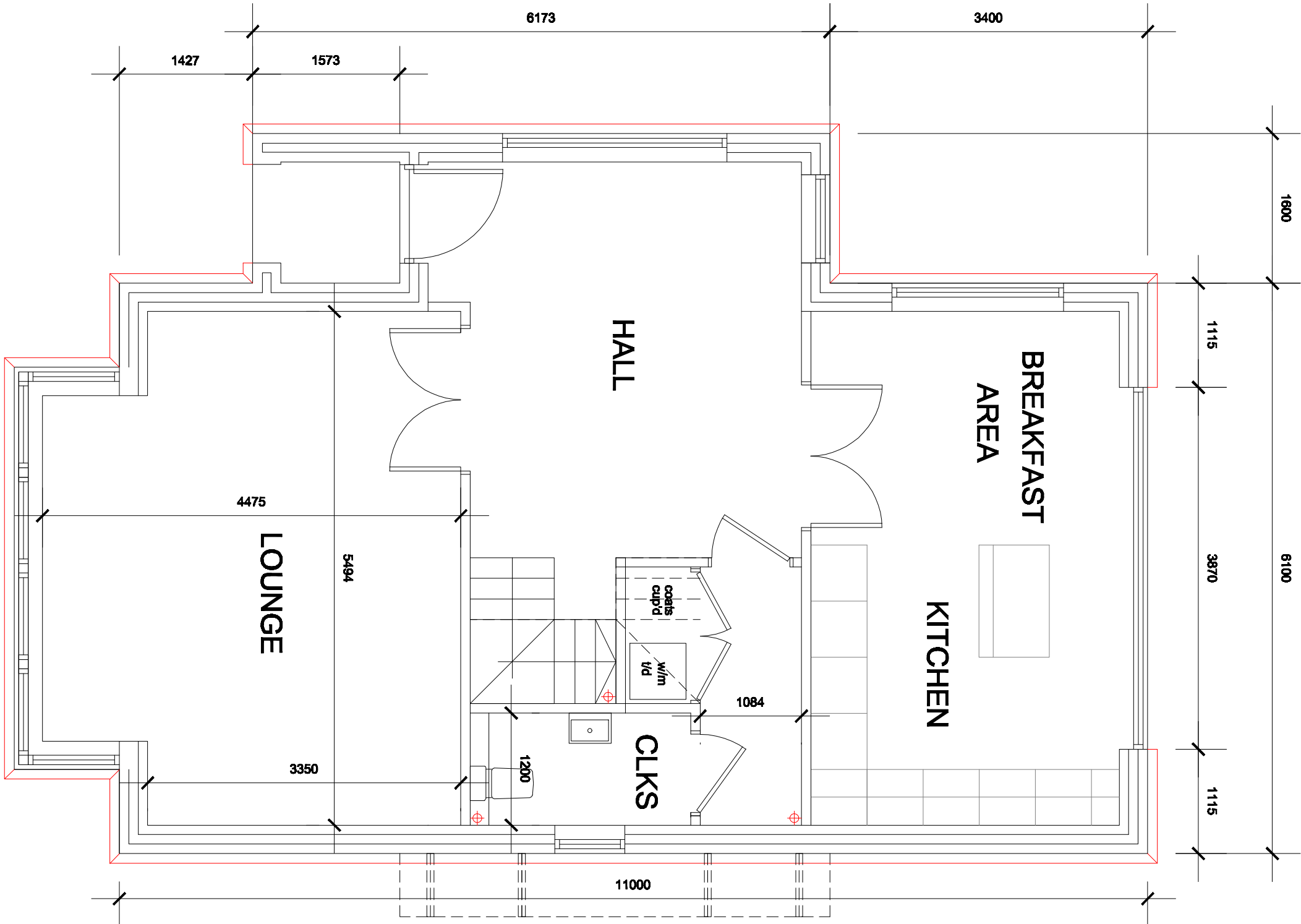
GROUND FLOOR PLAN 67m2
