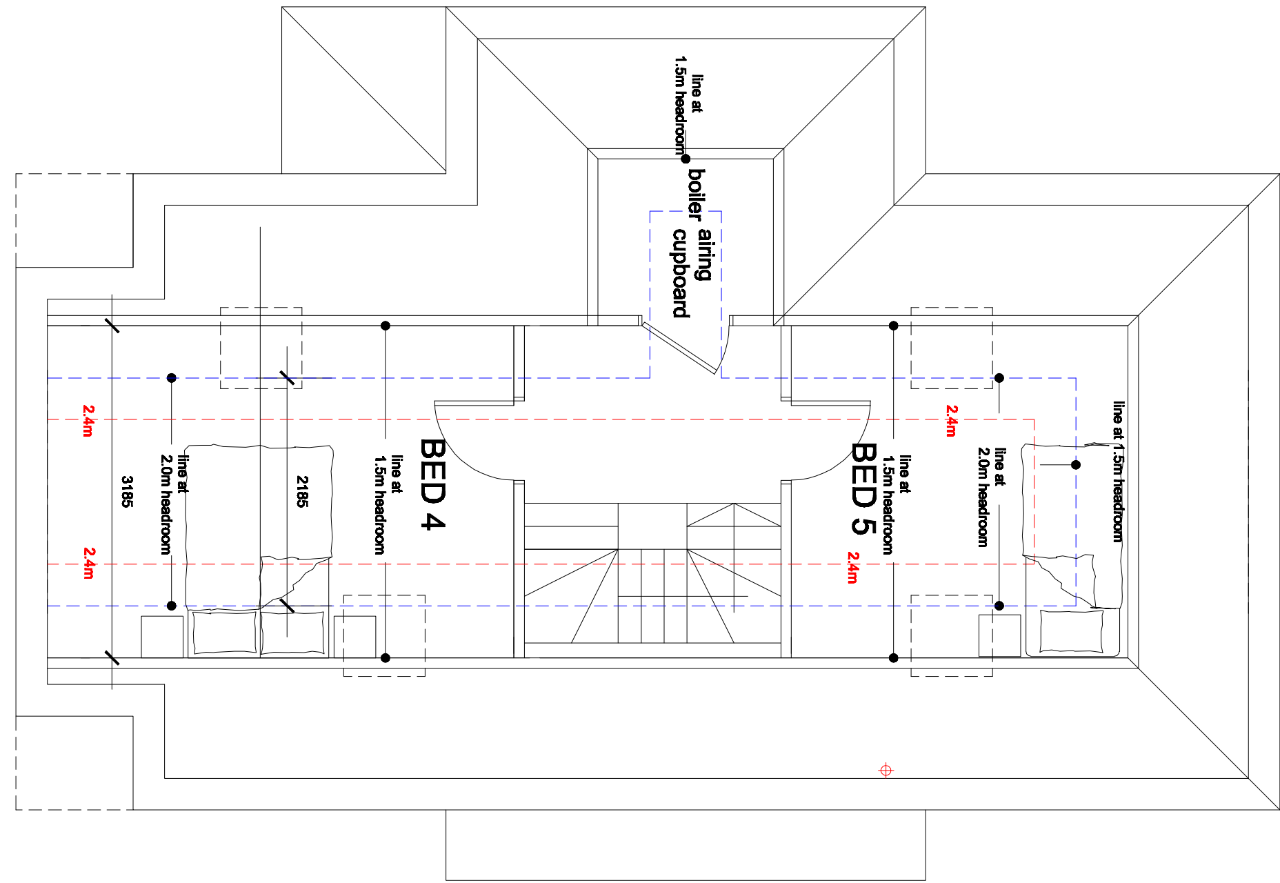
ROOF SPACE PLAN 36m2
