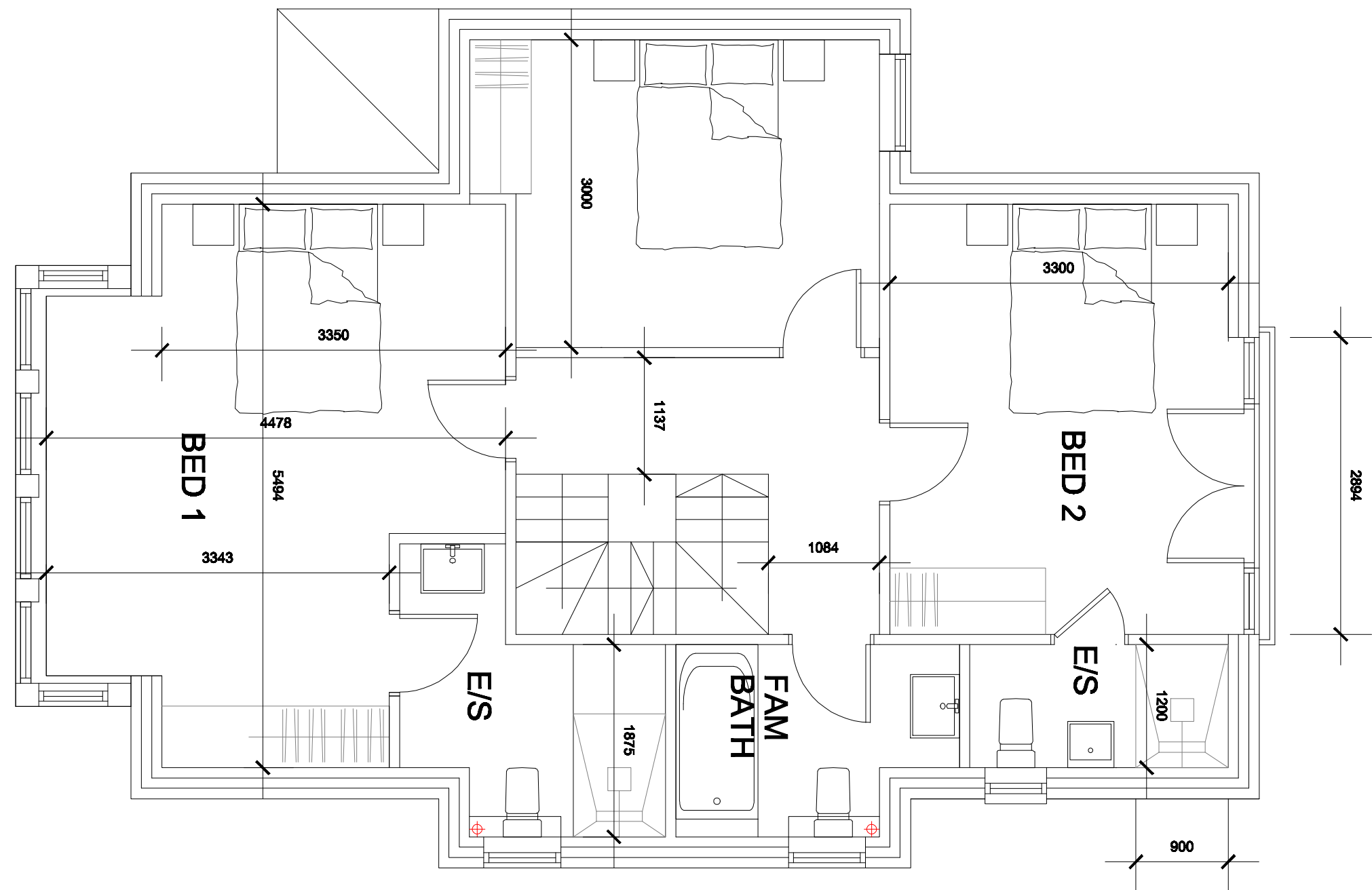
1ST FLOOR PLAN 70m2
